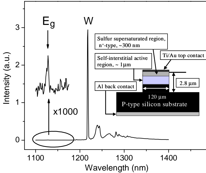
Fig. 1. Surface-emission photoluminescence spectrum of a sample without contacts at 7 K. The inset show the schematic of a Si light emitting diode (not to scale).
